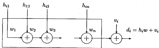
Fig. 1. Model for adaptive filtering.
