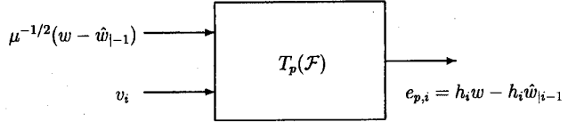
Fig. 2. Transfer operator from the unknown disturbances \{\mu^{-1/2}(w - \hat{w}_{|i-1}), \{v_j\}_{j=0}^{\infty}\} to the prediction errors \{e_{p,j}\}_{j=0}^{\infty} . Likewise for T_f(\mathcal{F}) .
