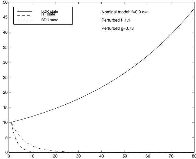
FIG. 6.1. Comparison of the LQR, \mathcal{H}_\infty , and BDU designs.
