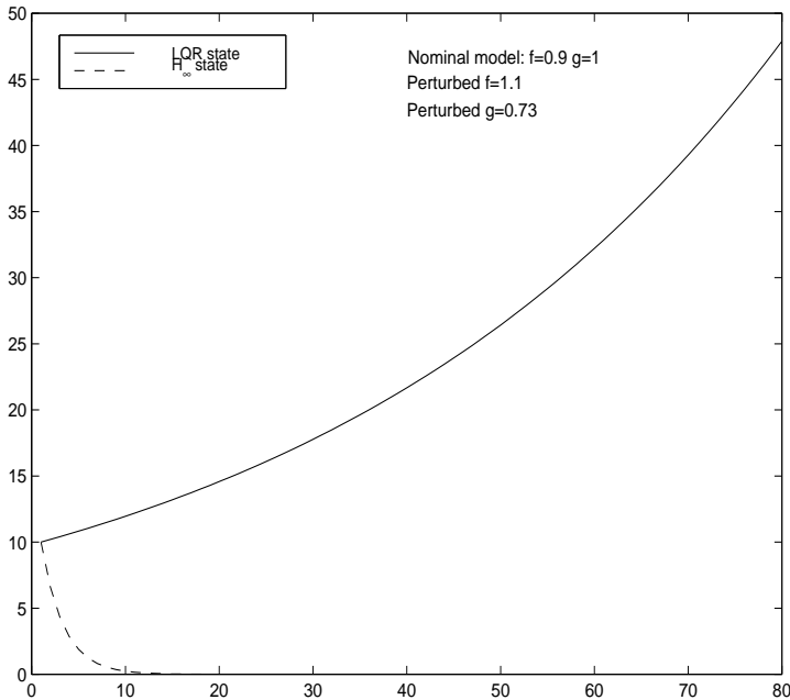
FIG. 3.4. \mathcal{H}_{\infty} control of the perturbed plant.
