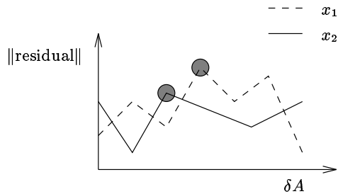
FIG. 4.1. Two illustrative residual-norm curves.
