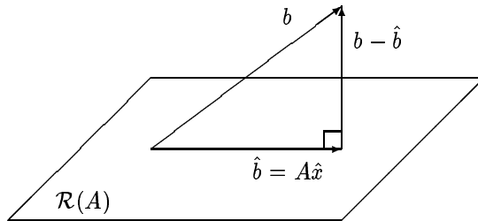
FIG. 2.1. The residual vector is orthogonal to \mathcal{R}(A) .
