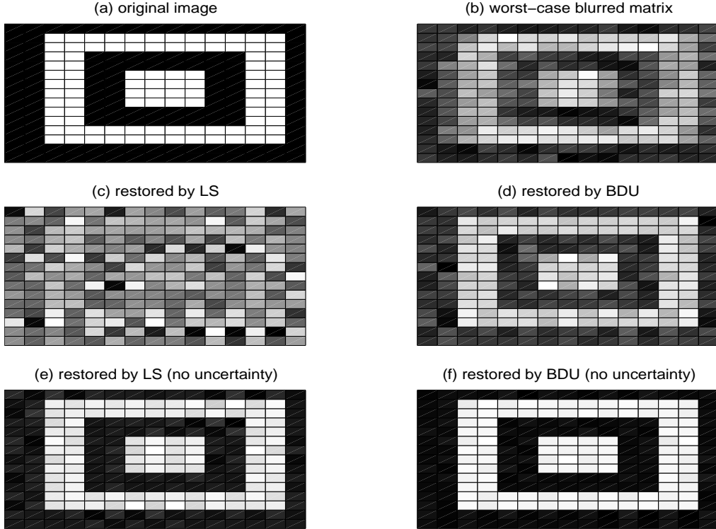
FIG. 5.4. Image processing example revisited.
