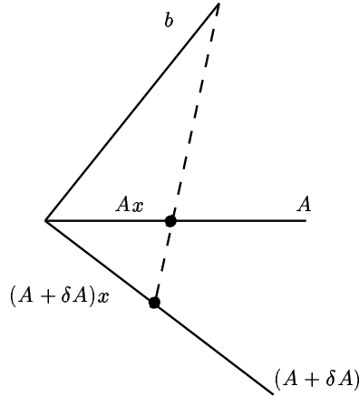
FIG. 5.2. The residual vectors [(A + \delta A)x - b] and Ax - b are collinear for any \delta A that attains the maximum residual norm.
