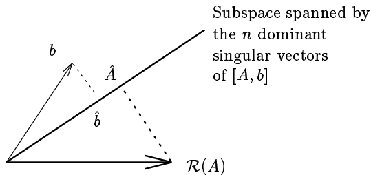
FIG. 3.1. Construction of the TLS solution.
