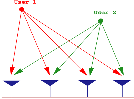
FIG. 7.1. Spatial-processing with multiple users.
