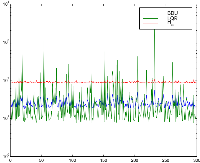
FIG. 6.2. 300 random runs with \eta_f = 0.2 and \eta_g = 0.27 .
