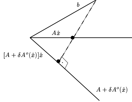
FIG. 5.3. Orthogonality condition for BDU estimation.
