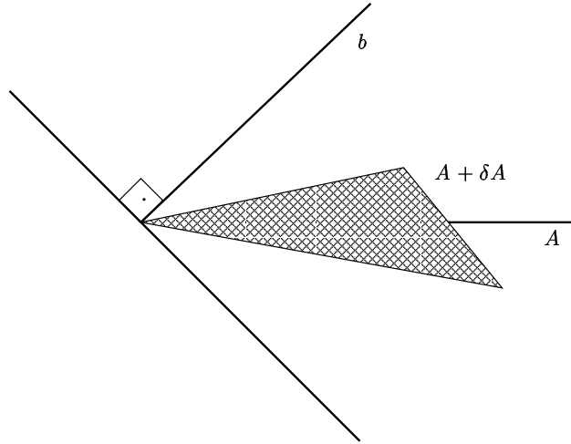
FIG. 5.1. A depiction of the case \eta < \frac{\|A^T b\|}{\|b\|} .
