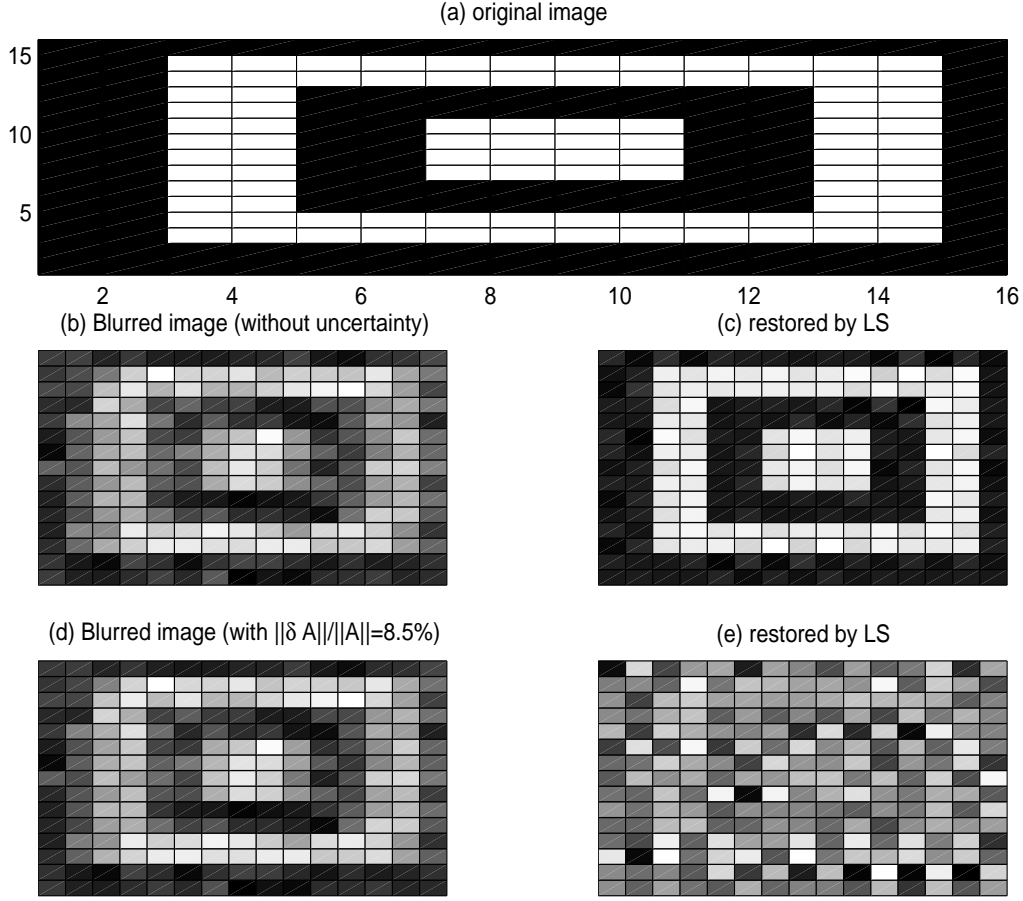
FIG. 2.2. Recovering an image from its blurred versions.
