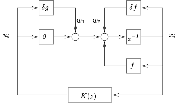
FIG. 3.2. Block diagram representation of the perturbed state-equation.
