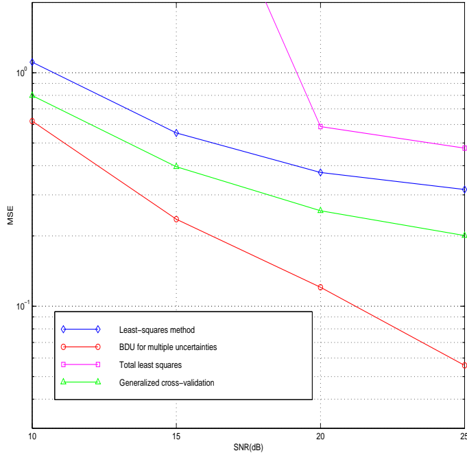
FIG. 7.2. 4PAM modulation, N = 4000 runs, \eta_x \approx 7\% , \eta_\theta \approx 22\% .
