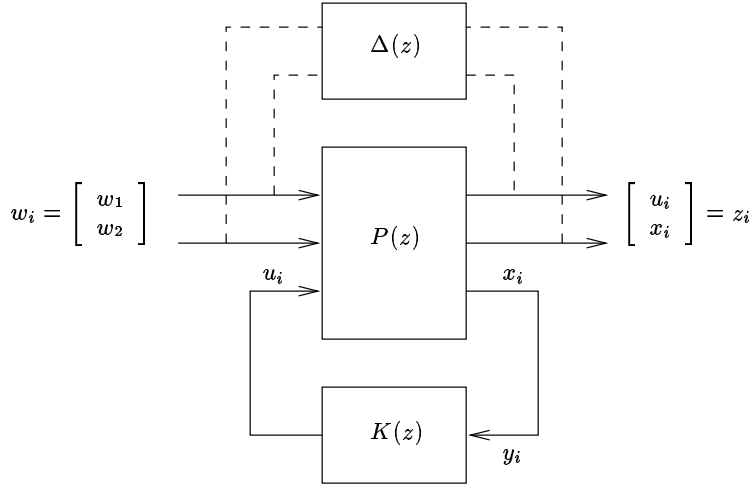
FIG. 3.3. Representation of the perturbed state-equation in standard form.
