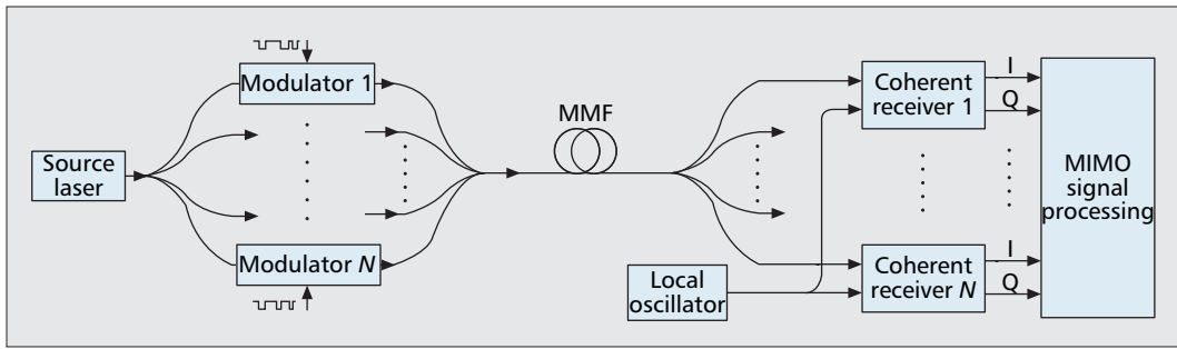
■ Figure 2. A coherent optical MIMO link.
