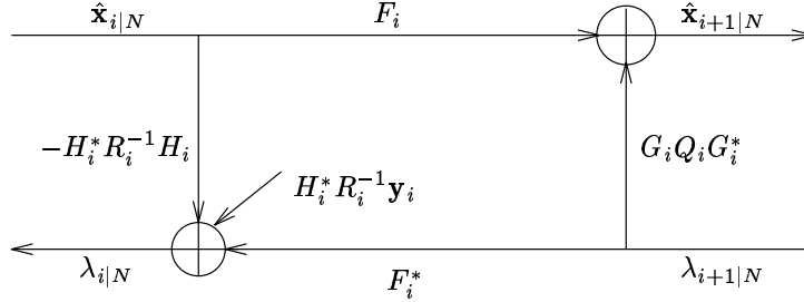
Figure 1: A scattering layer for the fixed-interval smoothing problem.
