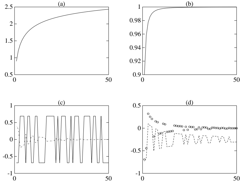
Figure 1: H^\infty norm of transfer operator as a function of the number of observations for (a) RLS, and (b) LMS. The true output and the worst case disturbance signal (dotted curve) for RLS are given in (c). The predicted errors for the RLS (dashed) and LMS (dotted) algorithms corresponding to this disturbance are given in (d). The LMS predicted error goes to zero while the RLS predicted error does not.
