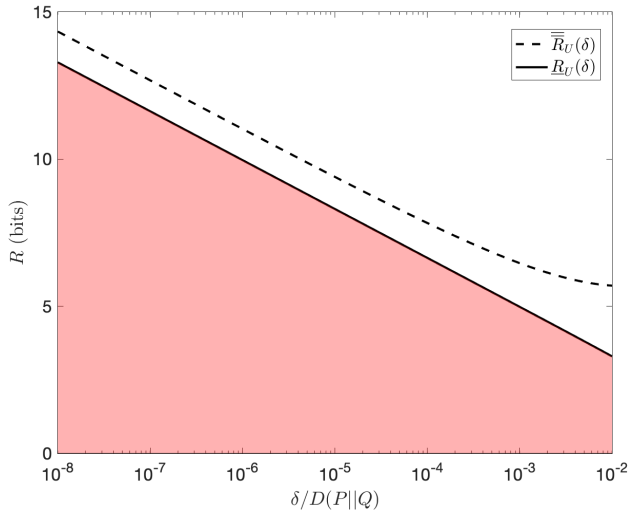
Fig. 2. Plot of the required number of bits ( R ) versus \delta in logarithmic scale at high rate regime for the same Gaussian U and with same \underline{R}_U(\delta) given in Fig. 1. The dashed curve is the upper bound \overline{R}_U(\delta) in (24) obtained with a lattice quantization scheme. No point in the shaded region is achievable. The difference of 1.047 bits is visible for low \delta .
