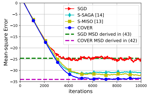
Fig. 2. Convergence comparison between SGD, S-SAGA, S-MISO and COVER.
