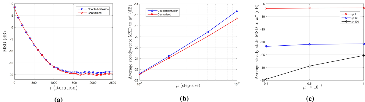
Fig. 2: (a) MSD learning curve for \mu = 0.005 and \eta = 10 . (b) MSD for different values of step size \mu with \eta = 10 . (c) Average steady-state error to w^\circ for different values of \eta and \mu .
